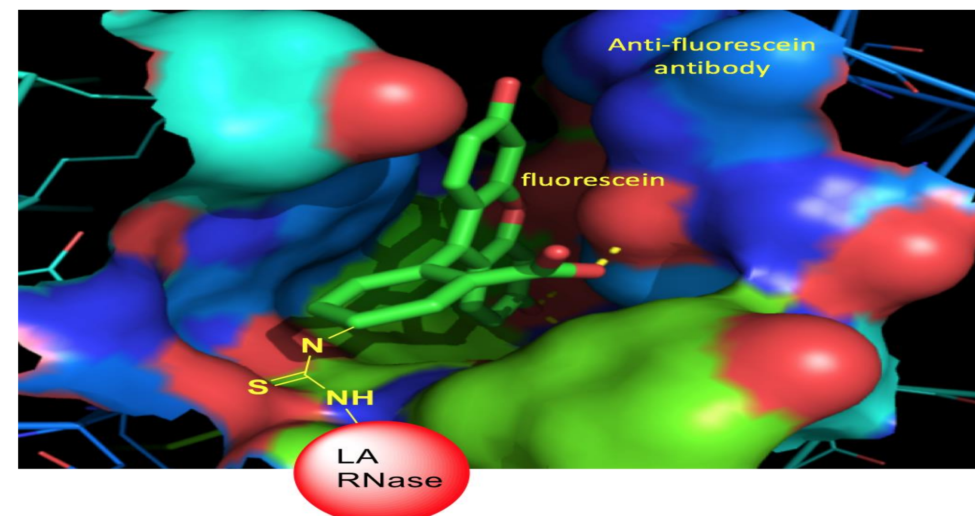
Figure 5. Covalent binding of modified RNase with FITC to anti-fluorescein antibody.
