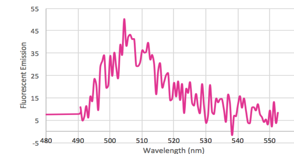
Figure 4. Difference emission spectrum (fluorescence intensity without antibody - fluorescence intensity + antibody) for Figure 3 showing quenching of fluorescein fluorescence by anti-fluorescein antibody.
