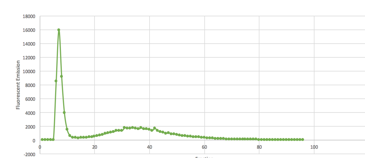
Figure 1. Size exclusion chromatography of fluorescein-labeled RNase as measured by fluorescence emission ( \lambda excitation = 482 nm, \lambda emission = 490-510 nm). Peak 1 is modified protein and peak 2 is excess FITC.
