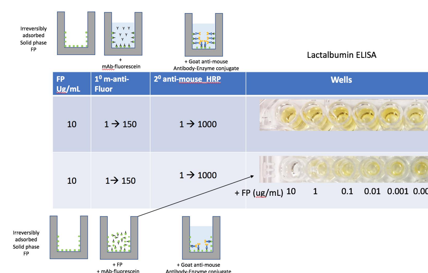
Figure 5. ELISA assay results of bovine lactalbumin with varying concentrations of fluorescently labeled bovine lactalbumin (row 2) compared to control group without fluorescently labeled bovine lactalbumin (row 1).
