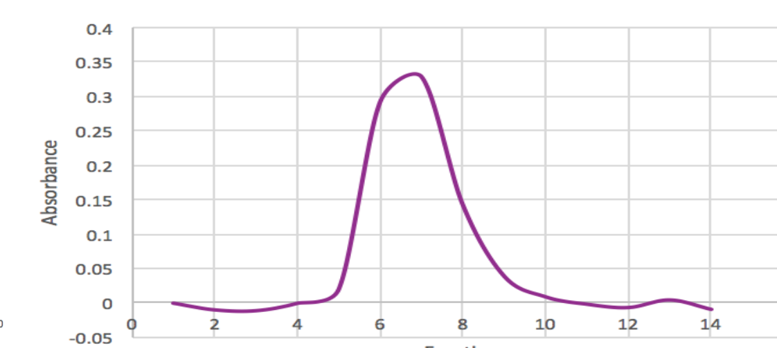
Figure 2. Size exclusion chromatography of fluorescein-labeled RNase as measured by absorbance at 280 nm (same fractions as in Figure 1).
