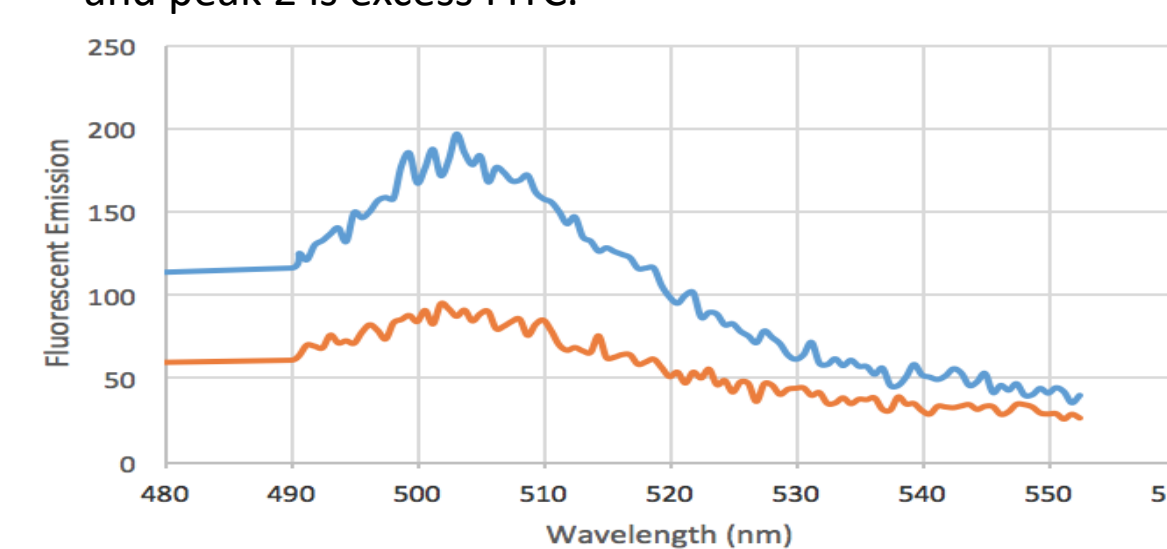
Figure 3. Comparison of emission spectrum in PBS buffer solution (pH 7.5, ) \lambda excitation = 482 nm • RNase + anti-fluorescent antibody (orange) • RNase - anti-fluorescent antibody (blue)
